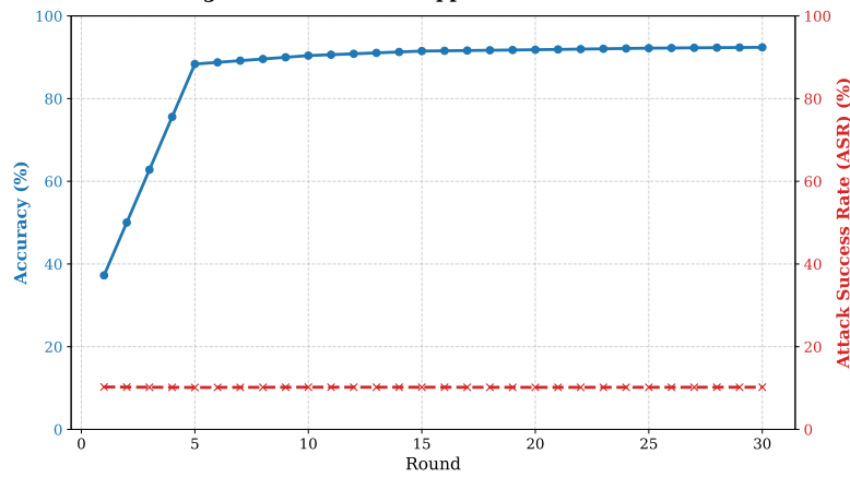
Fig. 6. Evolutionary curves of global computational convergence Accuracy and Backdoor Attack Success Rate (ASR).
